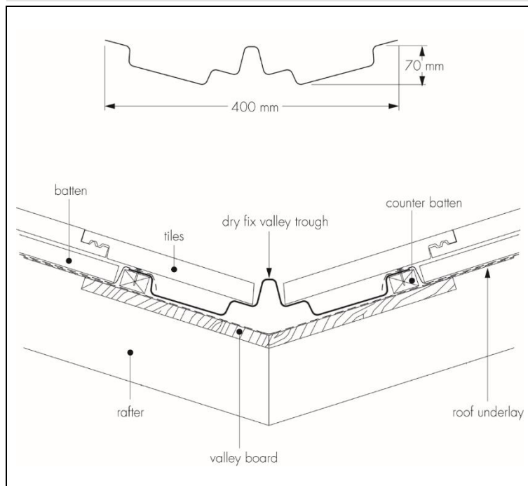
Figure 4 Over Batten Dry Fix Valley Troughs — 0645627
