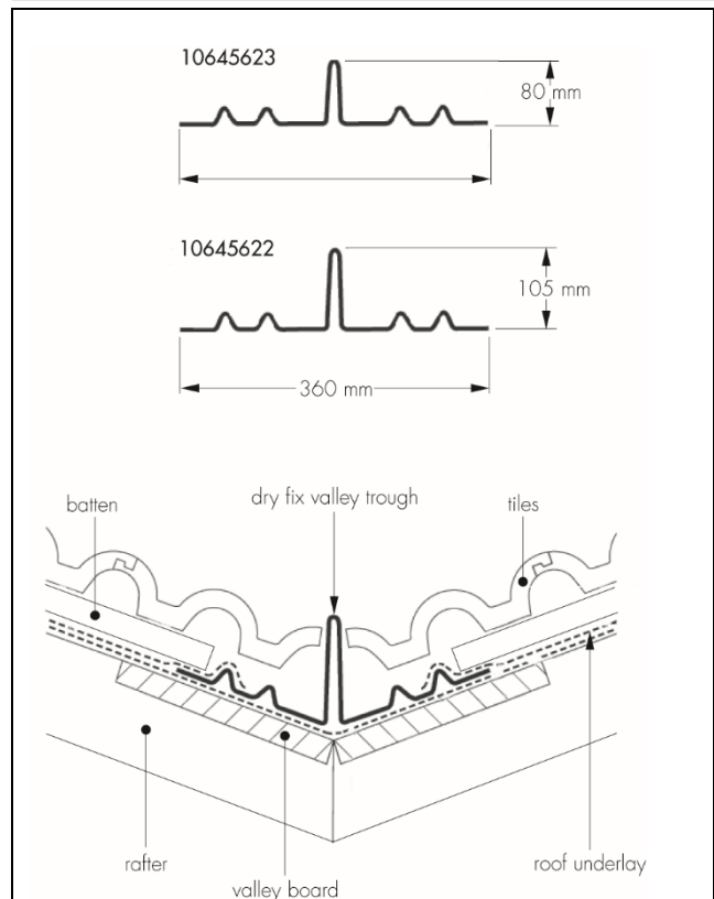
Figure 2 Dry Fix Valley Troughs
