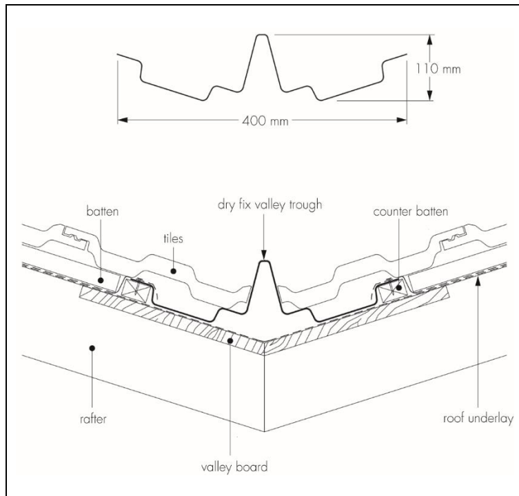
Figure 3 Over Batten Dry Fix Valley Troughs — 10645628
